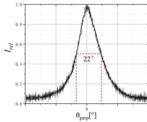
Beam spread
